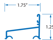
Clean Track Detail
